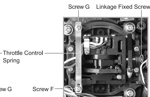
Left throttle set
