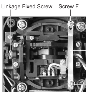
Right throttle set
